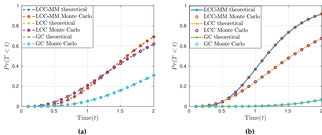
Figure 2. Per-iteration completion time statistics; (a) K = 6, r = 3 , and (b) N = K, r = 5 .
