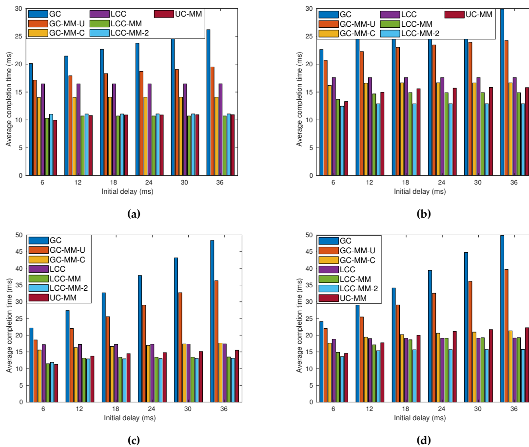
Figure 7. Average completion time analysis for GC, GC-MM-U, GC-MM-C, LCC, LCC-MM, LCC-2 and UC-MM schemes with random fixed initial delay and exponential communication delay; (a) r = 6 , p = 0.2 and \mu = 2 , (b) r = 6 , p = 0.2 and \mu = 4 , (c) r = 6 , p = 0.4 and \mu = 2 , and (d) r = 6 , p = 0.4 and \mu = 4 .
