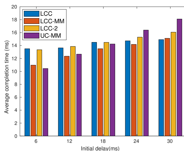
Figure 13. Performance under uncorrelated delay.
