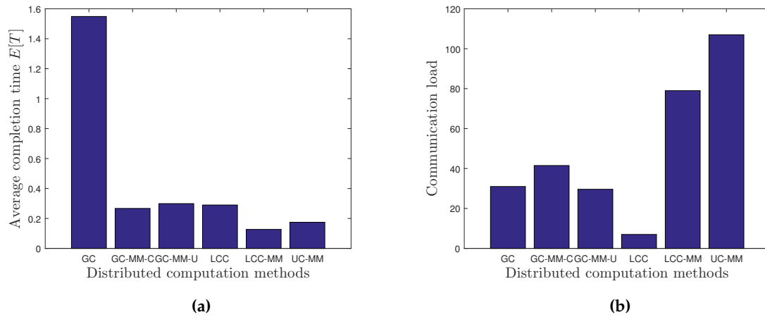
Figure 3. Per-iteration completion time and communication load statistics; (a) average completion time performance, and (b) communication load performance.
