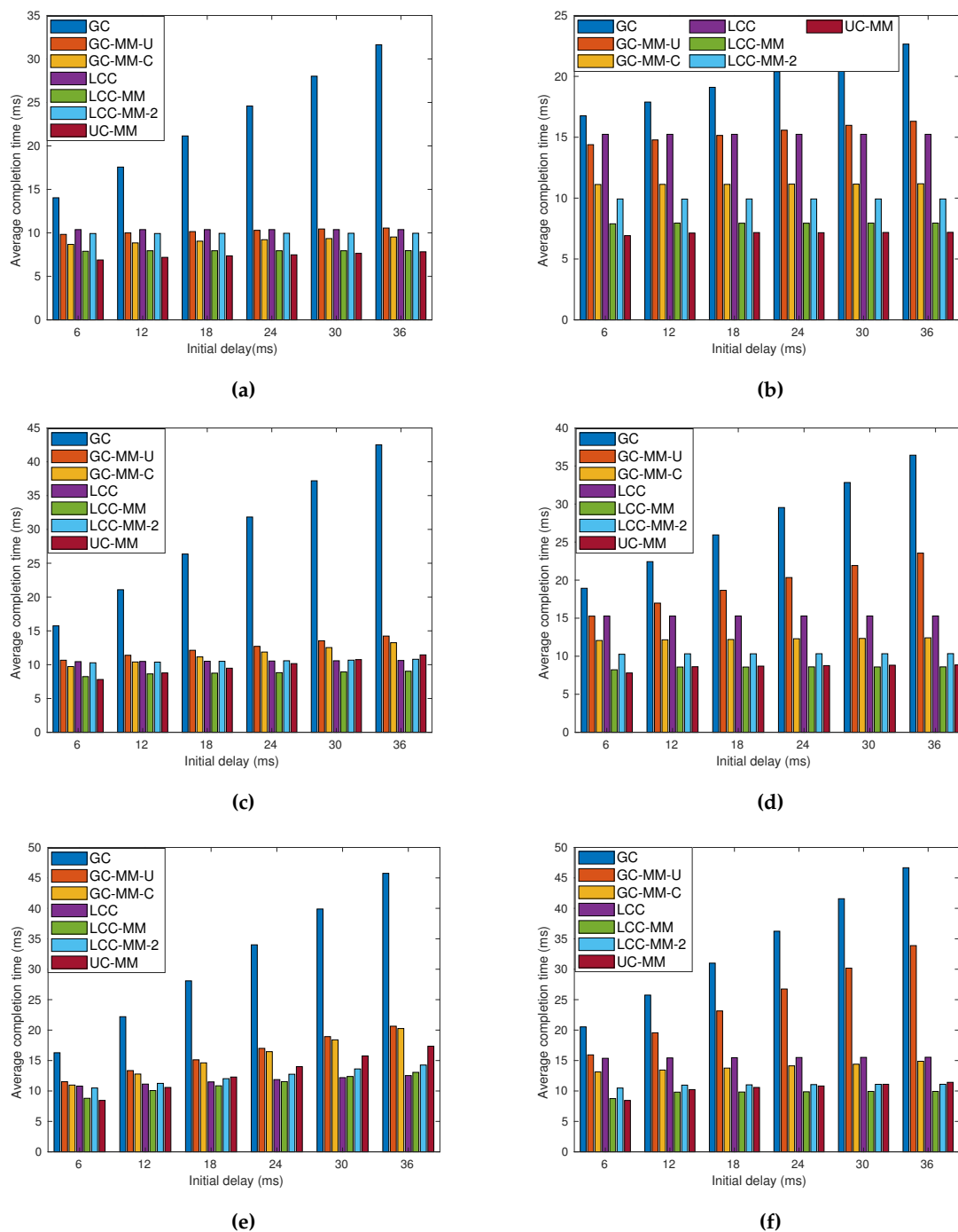
Figure 5. Average completion time analysis for GC, GC-MM-U, GC-MM-C, LCC, LCC-MM, LCC-2 and UC-MM schemes with random fixed initial delay; (a) r = 4 and p = 0.2 , (b) r = 6 and p = 0.2 , (c) r = 4 and p = 0.3 , (d) r = 6 and p = 0.3 , (e) r = 4 and p = 0.4 , and (f) r = 6 and p = 0.4 .
