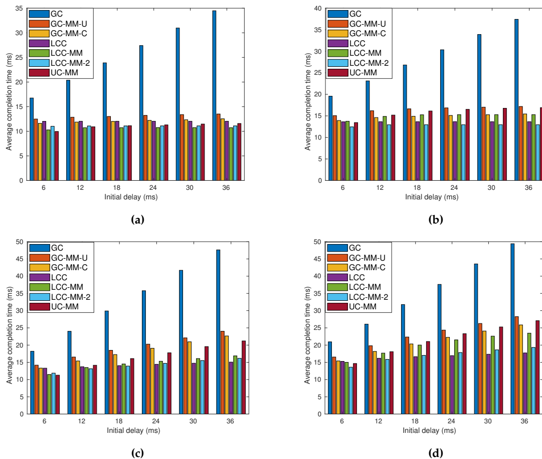
Figure 6. Average completion time analysis for GC, GC-MM-U, GC-MM-C, LCC, LCC-MM, LCC-MM-2 and UC-MM schemes with random fixed initial delay and exponential communication; (a) r = 4 , p = 0.2 , \mu = 2 , (b) r = 4 , p = 0.2 , \mu = 4 , (c) r = 4 , p = 0.4 , \mu = 2 , and (d) r = 4 , p = 0.4 , \mu = 4 .
