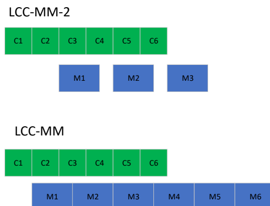
Figure 8. Overlapping communication and computation, green and blue blocks illustrate the computation and the communication steps, respectively.
