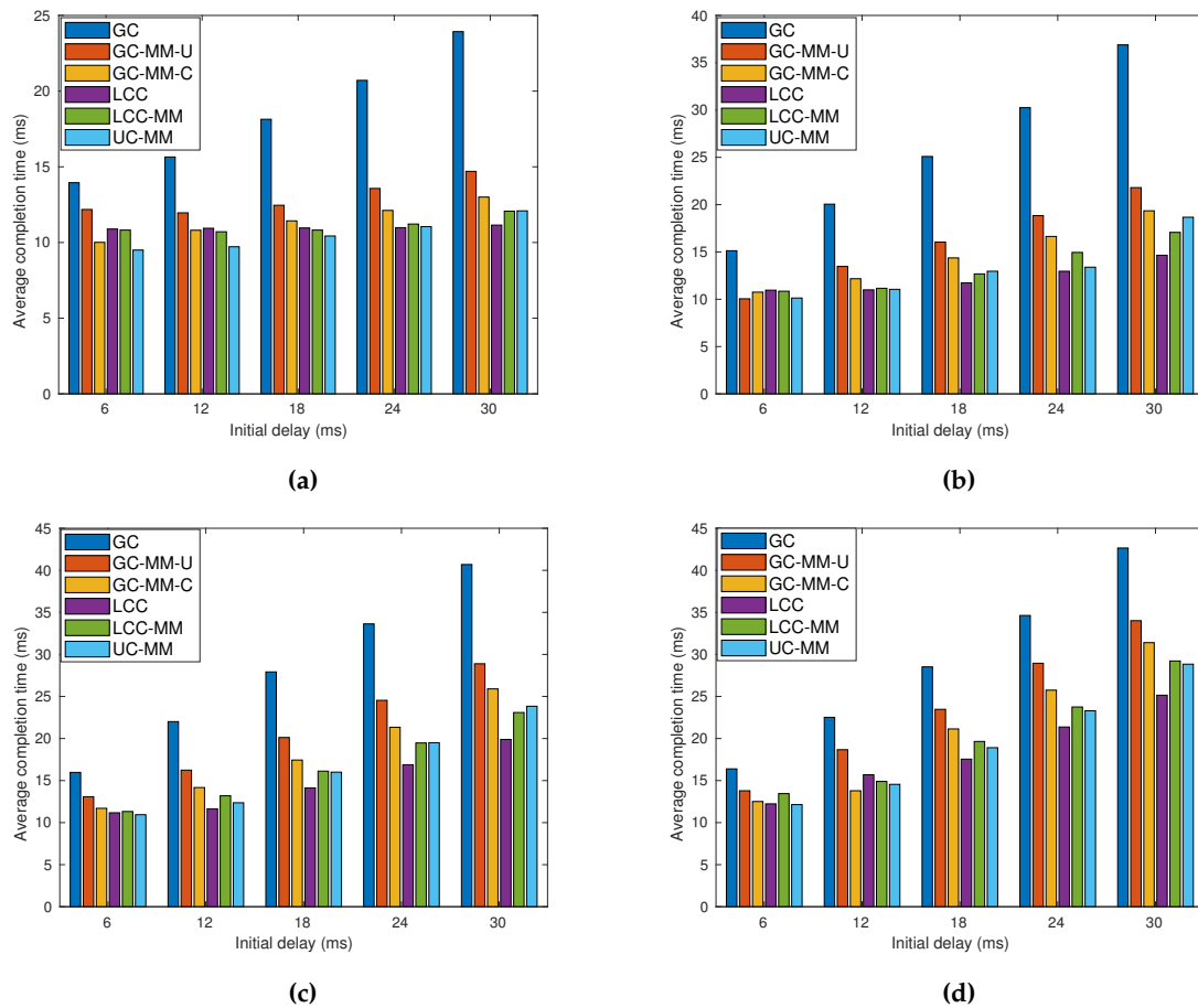
Figure 10. Per-iteration completion time for different schemes with r = 3 ; (a) p = 0.1 , (b) p = 0.2 , (c) p = 0.3 , and (d) p = 0.4 .
