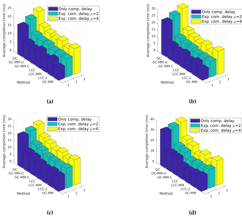
Figure 9. Per-iteration completion time for different schemes with r = 4 ; (a) failure probability p=0.2 , initial delay 12 ms, (b) failure probability p=0.2 , initial delay 24 ms, (c) delay probability p=0.4 , initial delay 12 ms, and (d) delay probability p=0.4 , initial delay 24 ms.
