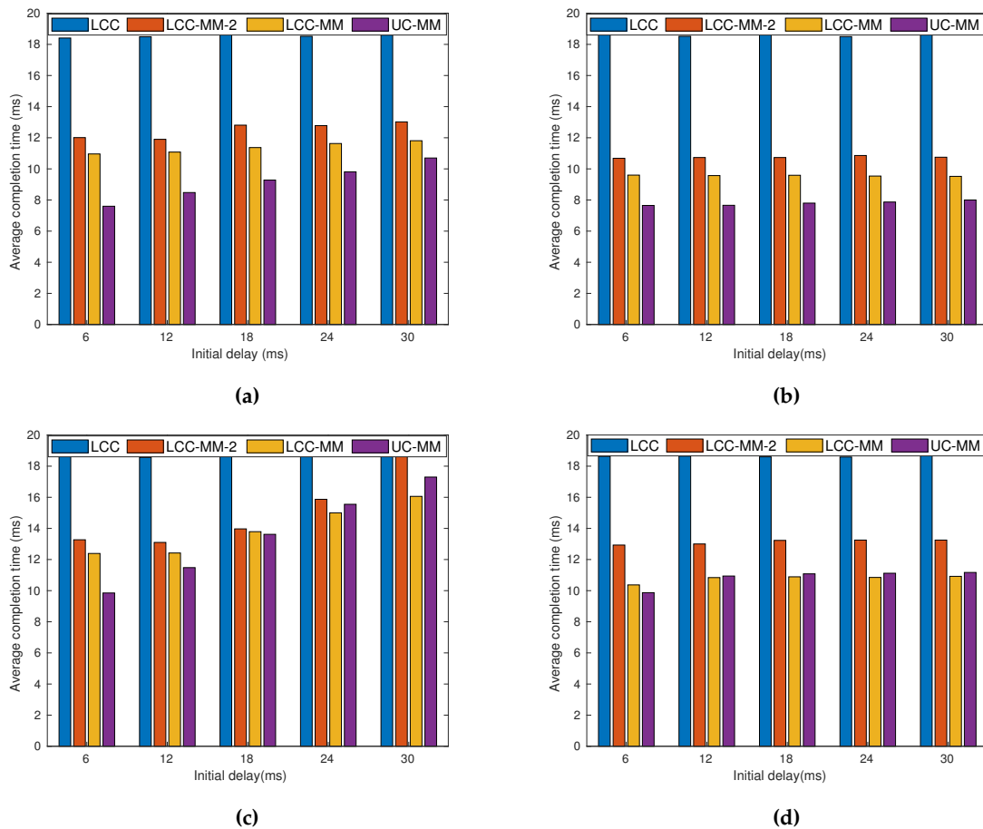
Figure 14. Per-iteration completion time for different schemes with r = 6 ; (a) correlated delay, p = 0.1 , (b) uncorrelated delay, p = 0.1 (c) correlated delay, p = 0.3 , and (d) uncorrelated delay, p = 0.3 .
