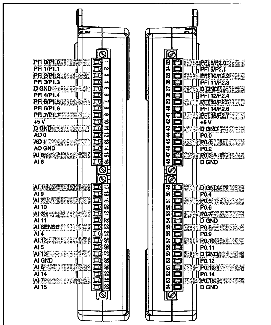
Figure A-3. USB-6212/6216 Screw Terminal Pinout
