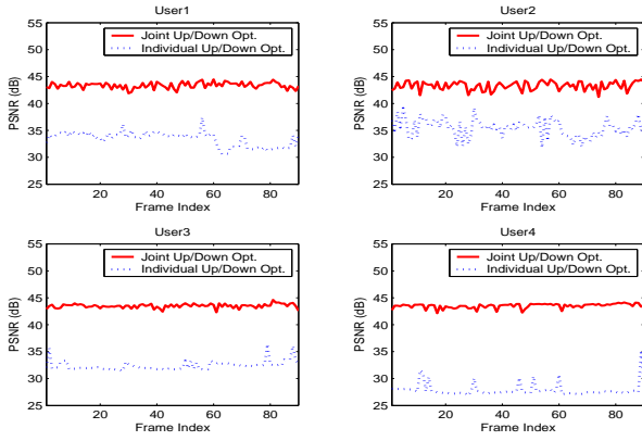
Fig. 3. Frame-by-frame PSNR result for User 1 to User 4.
