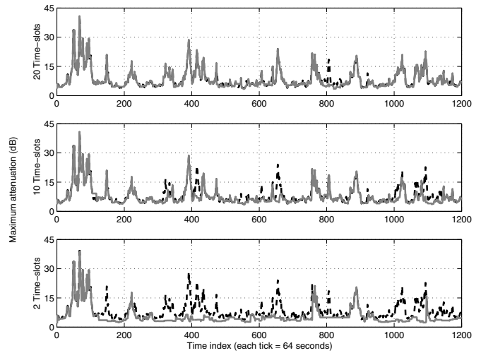
Fig. 3. Time-series plot of actual channel attenuation level (dashed-line) versus the level calculated at the NOC (solid-line) for a set of 200 users.
