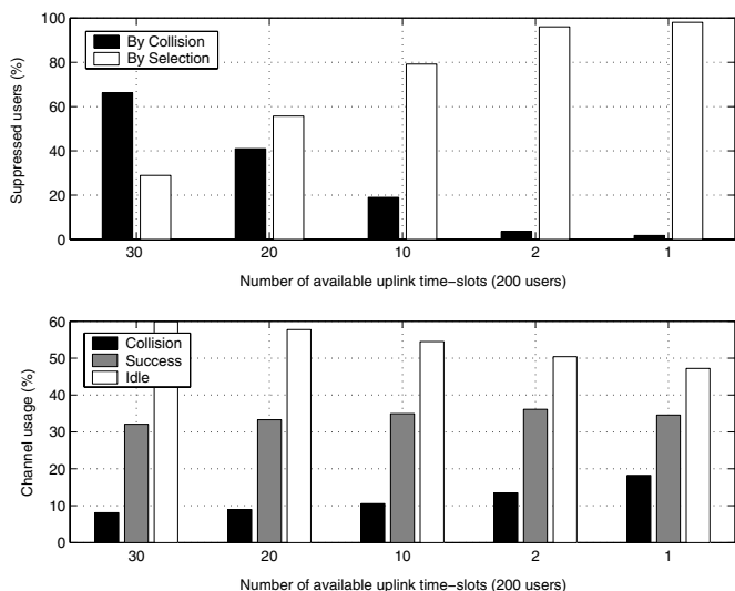
Fig. 4. (a) Fraction of the users suppressed by the FIS algorithm as a function of the number of available uplink time-slots (200 users). (b) Channel usage profile as a function of the number of available uplink time-slots (200 users).
