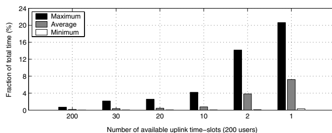
Fig. 6. Percentage of total time BER target is not met by a user as a function of number of available uplink time-slots (200 users).
