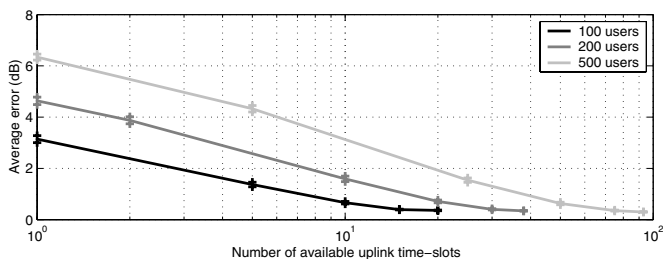
Fig. 5. Average error versus number of available uplink time-slots as a function of number of active users.
