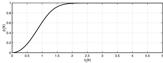
Fig. 2. Probability of transmission as a function of \Delta (dB).
