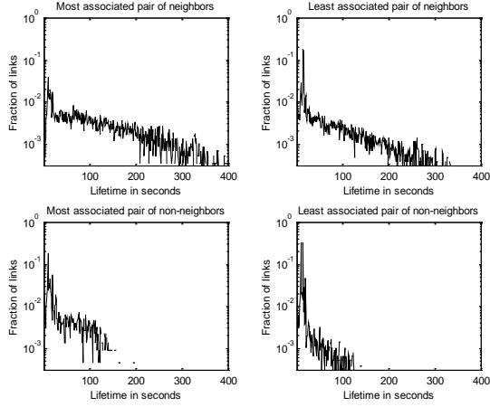
Figure 3. Probability that a link live t seconds
