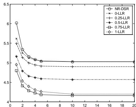
Figure 9. RREQ packets per second
