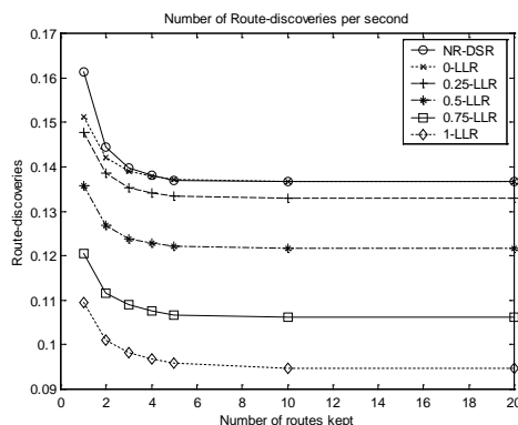
Figure 8. Route discoveries per second
