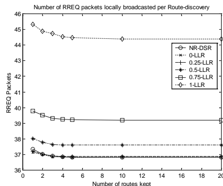
Figure 7. RREQ packets per route discovery
