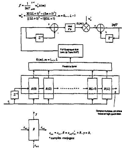
Figure 5: Systolic VLSI Structure of Carrier Frequency Offset Estimator
