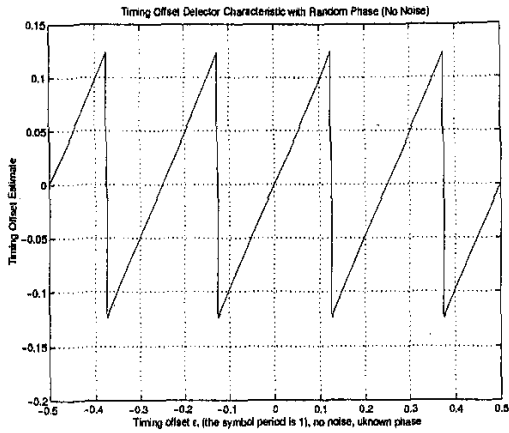
Figure 10: Timing Offset Estimate \hat{\epsilon} vs. Timing Offset \epsilon
