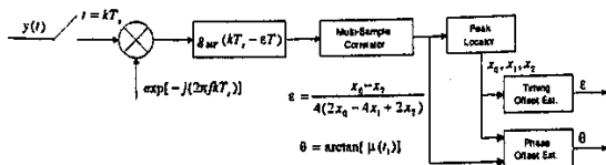
Figure 6: Joint Carrier Phase and Timing Offsets Estimator
