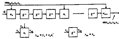
Figure 7: Multi-Sample Correlator
