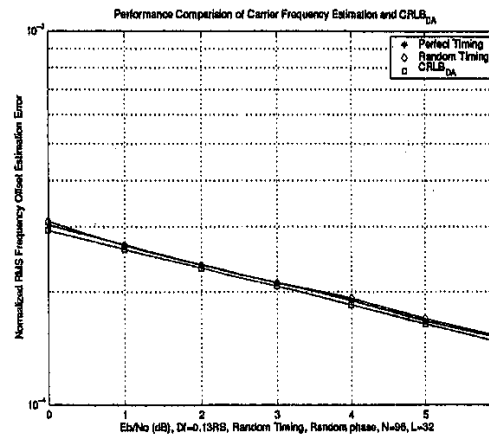
Figure 9: RMS Carrier Frequency Offset Estimation Error vs. CRLB_{DA}
