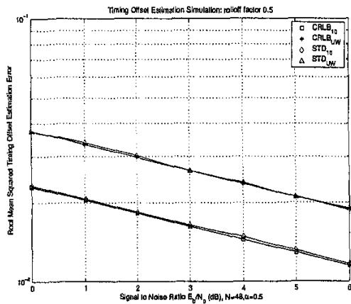
Figure 11: Timing Offset Estimation Performance (one zero pattern vs. UW pattern, \alpha = 0.5 )
