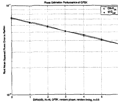
Figure 12: Phase Offset Estimation Performance (UW pattern, \alpha = 0.5 )
