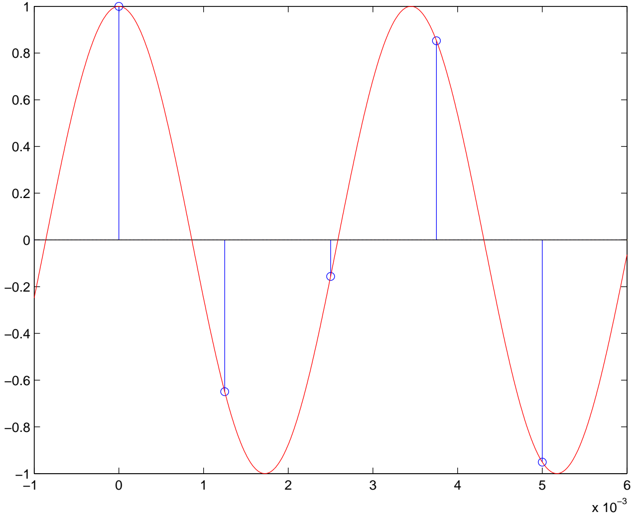
Interpolation by 290 Hz sinusoid
