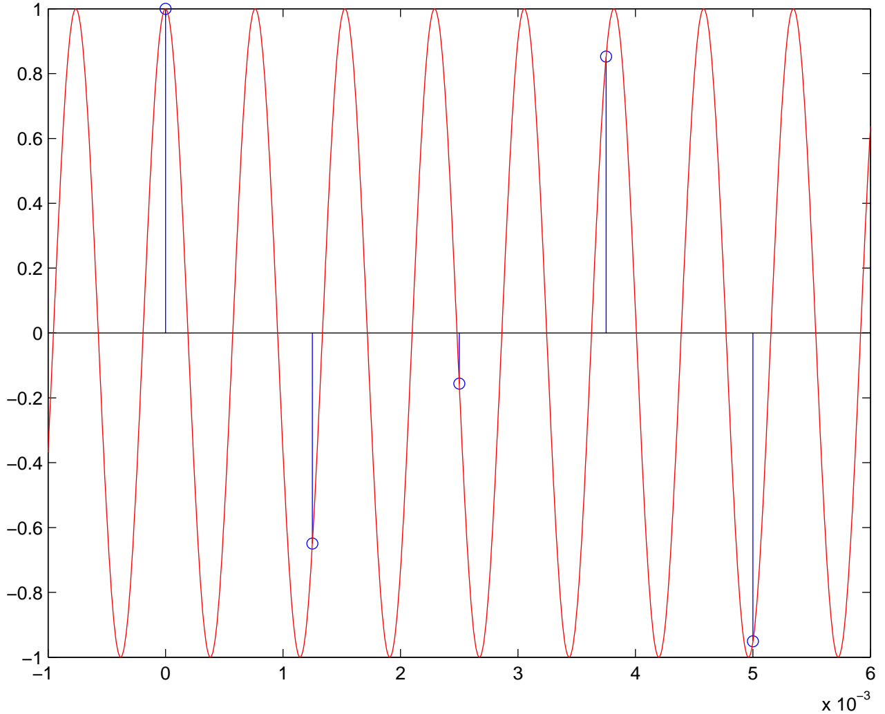
Interpolation by 1310 Hz sinusoid
