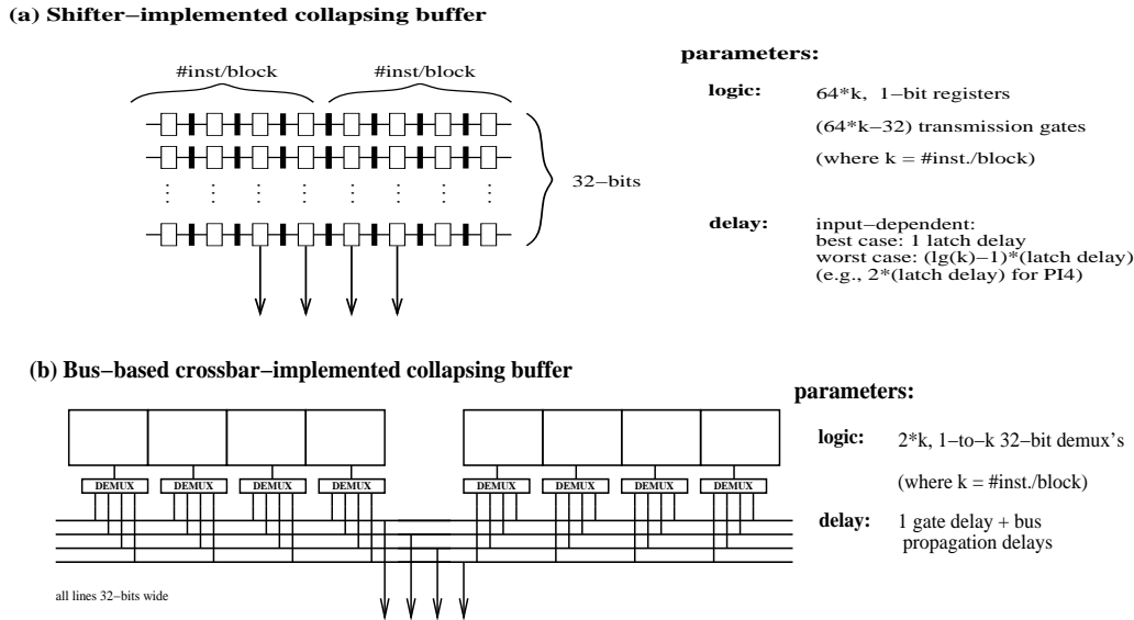
Figure 8: Design details of the collapsing buffer implemented (a) as a shifter, and (b) as a bus-based crossbar.
